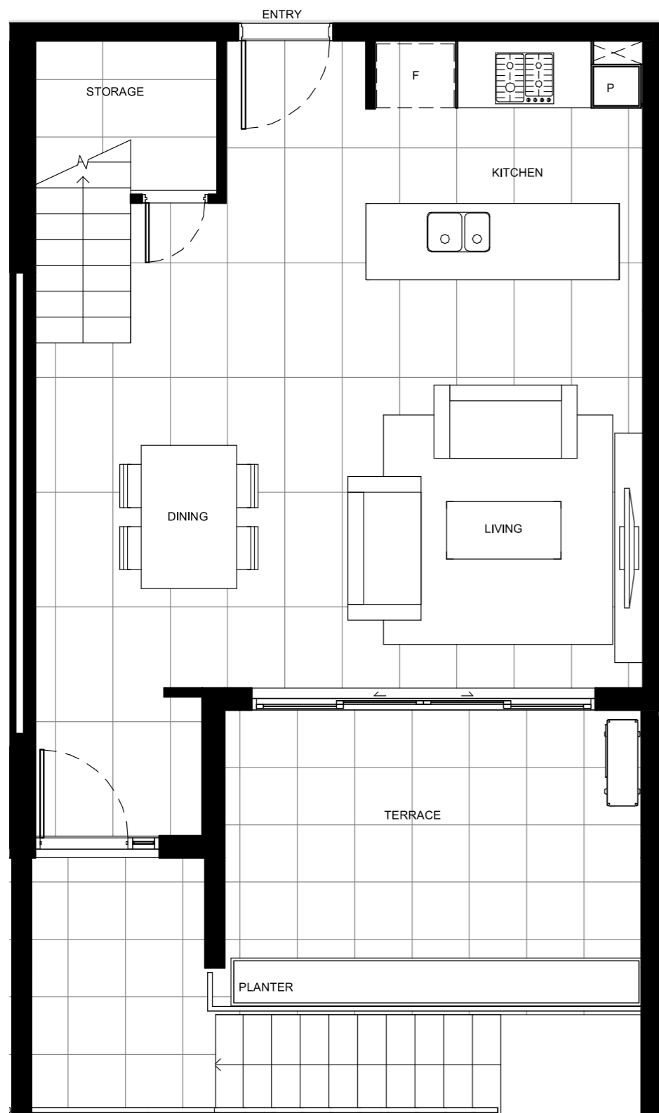
LEVEL 1
