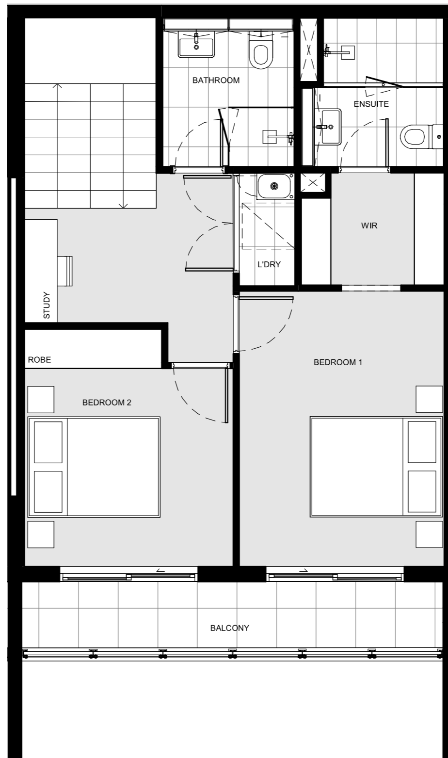
LEVEL 2
