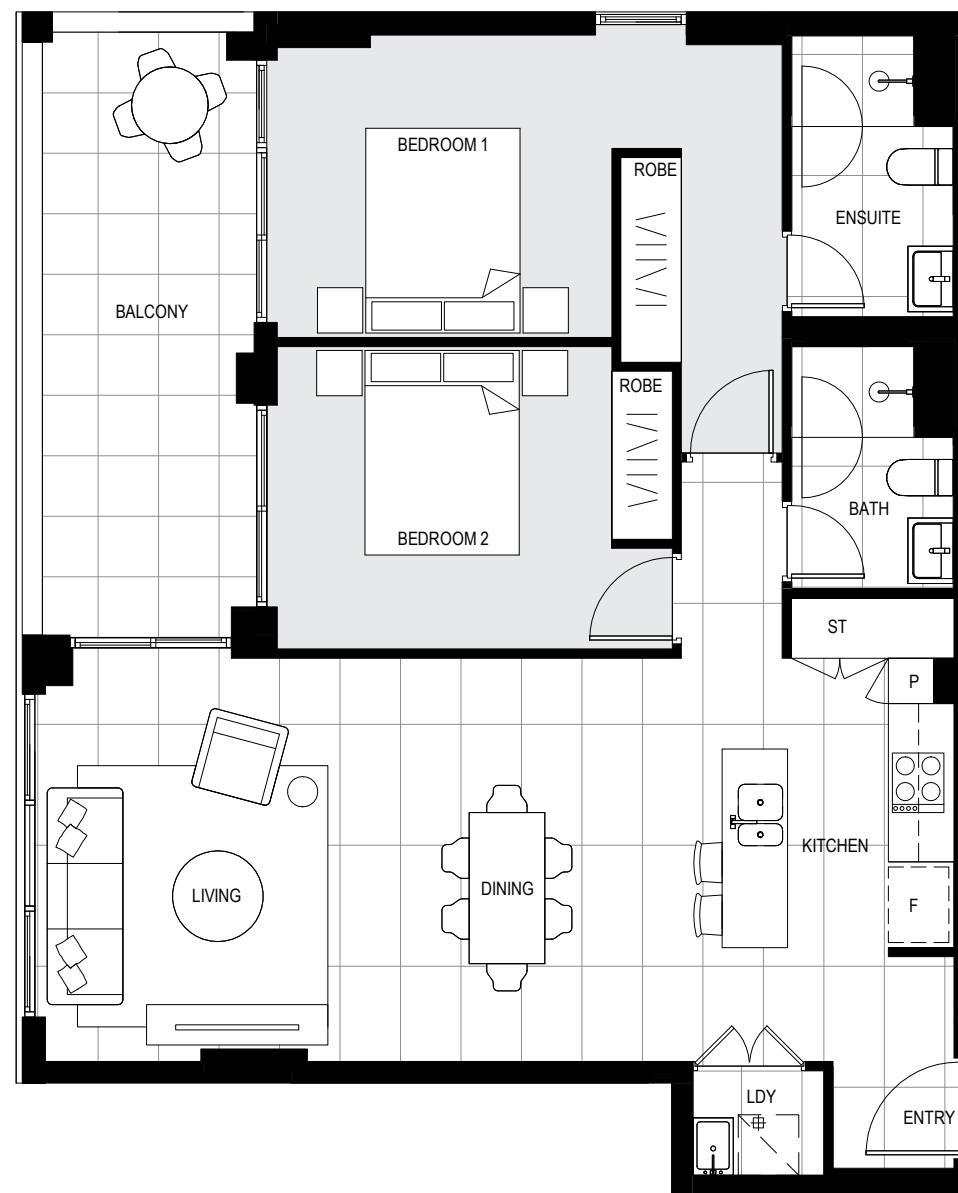
LEVEL 4
