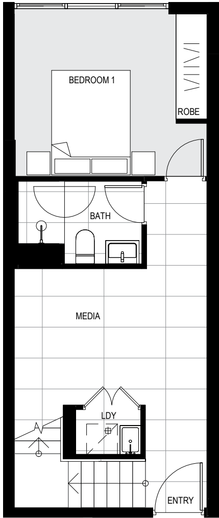
LEVEL 6
